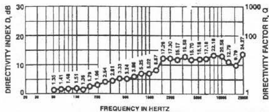
FIGURE 4 — Sx200 Directivity Response (anechoic environment)
