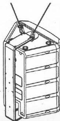
FIGURE 7 — Suspending the Sx200 Using Mb200 Installation Kit
