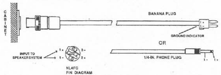
FIGURE 6 — Two-Conductor Cable Configurations for Sx200 Speaker System Using Neutrik Speakon® NL4FC Four-Pin Connector
