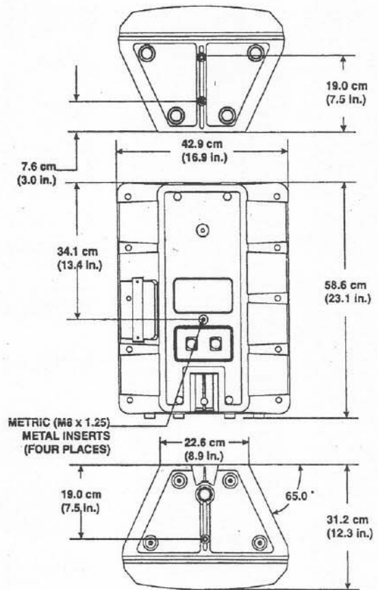
FIGURE 5 — Sx200 Dimensions
