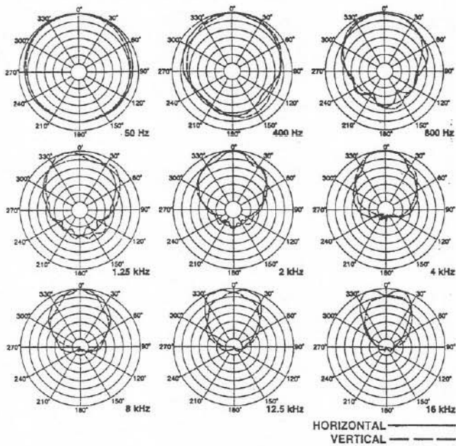
FIGURE 3 — Sx200 Beamwidth Response (anechoic environment)
