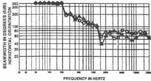
FIGURE 4 — Sx200 Directivity Response (anechoic environment)
