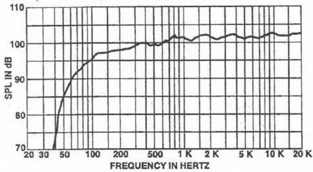
FIGURE 1 — Sx200 Frequency Response (1 watt/1 meter, anechoic environment)
